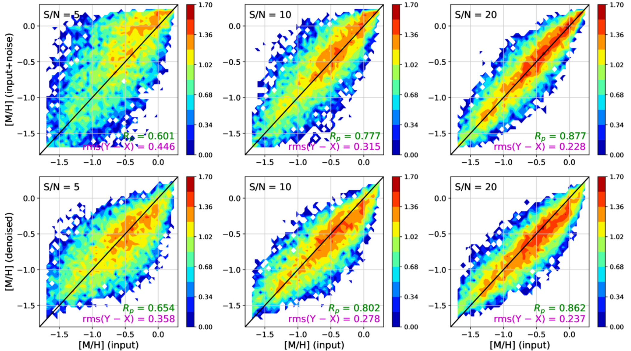
Figure 8. from Suk Kim et al 2026 Astron. J. 171 doi:10.3847/1538-3881/ae5a8c https://dx.doi.org/10.3847/1538-3881/ae5a8c © 2026. The Author(s). Published by the American Astronomical Society.
