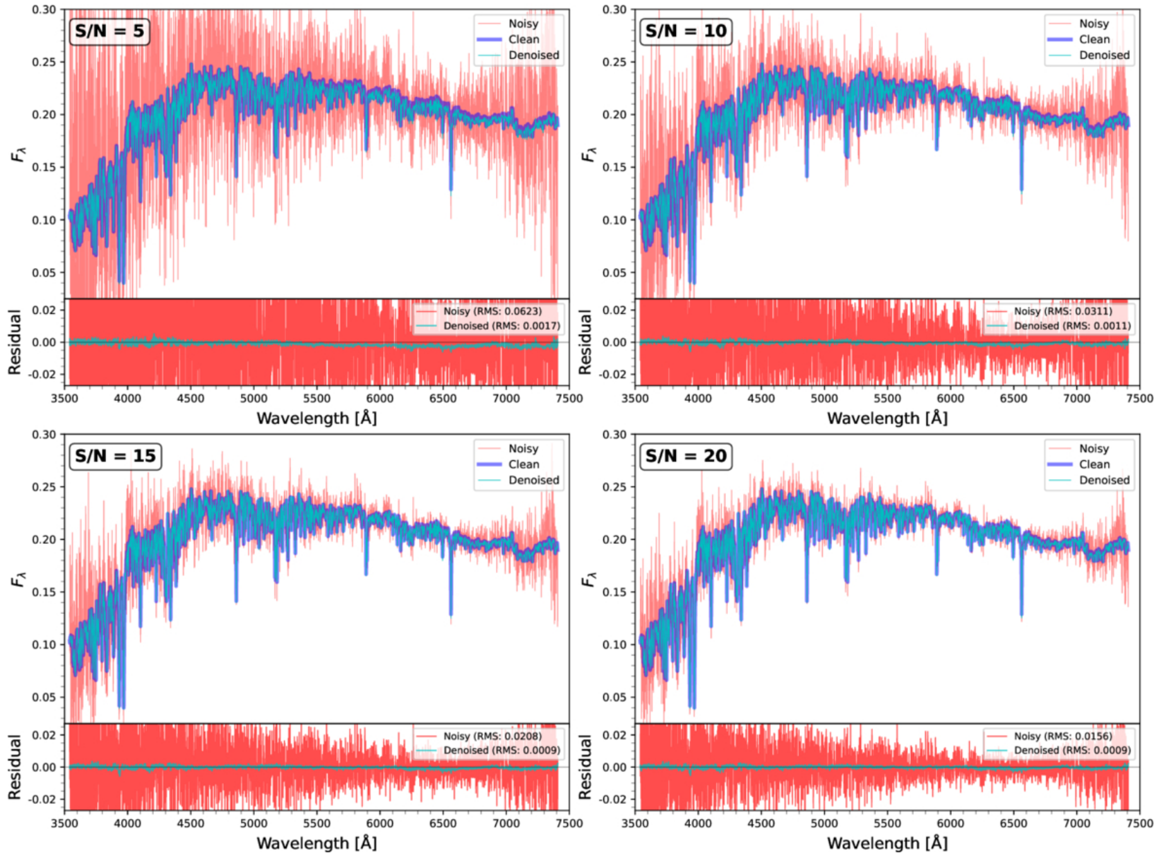
Figure 3. from Suk Kim et al 2026 Astron. J. 171 doi:10.3847/1538-3881/ae5a8c https://dx.doi.org/10.3847/1538-3881/ae5a8c © 2026. The Author(s). Published by the American Astronomical Society.
