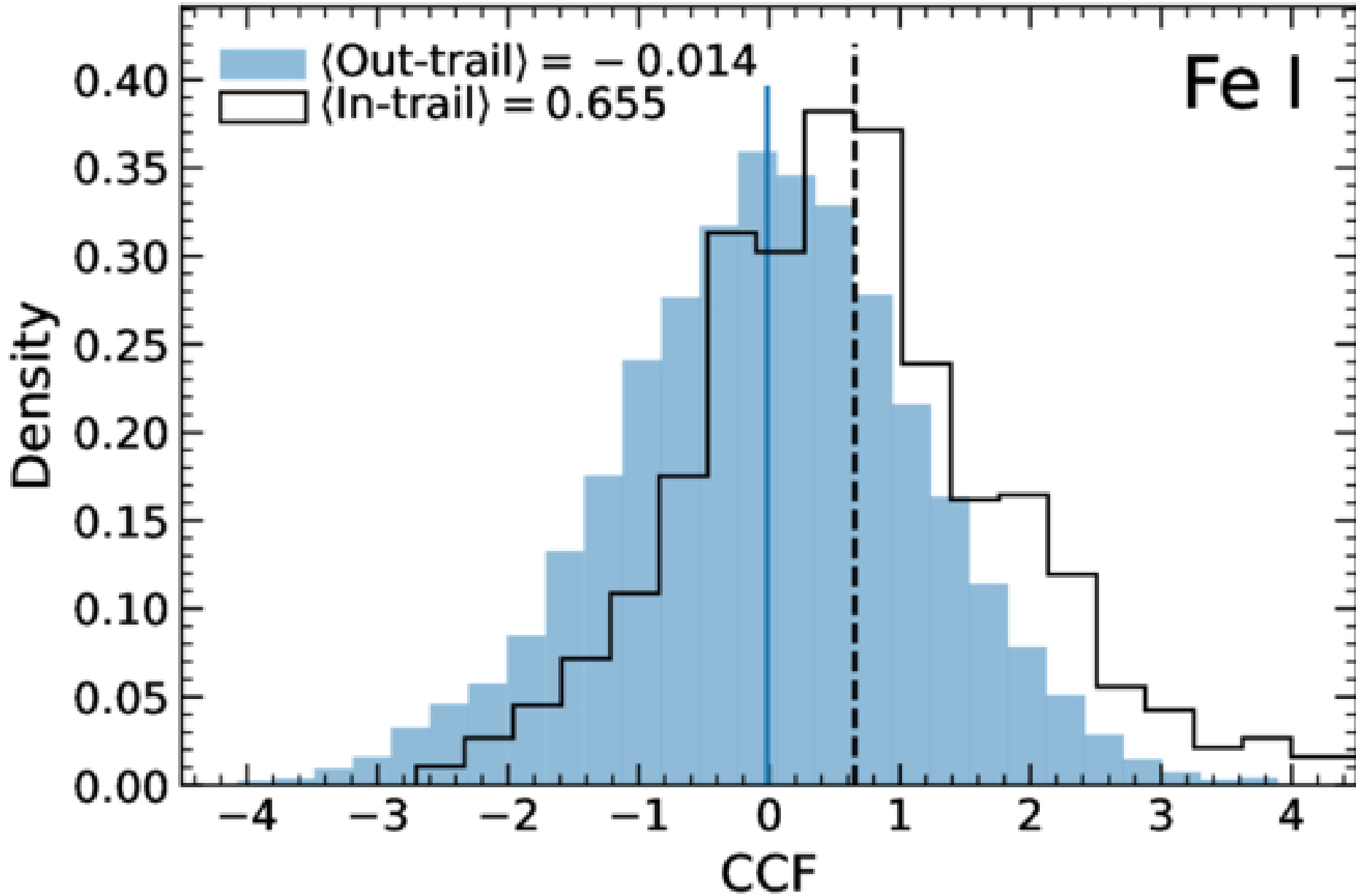
Figure 8. from James T. Sikora et al 2026 Astron. J. 171 doi:10.3847/1538-3881/ae5a29 https://dx.doi.org/10.3847/1538-3881/ae5a29 © 2026. The Author(s). Published by the American Astronomical Society.
