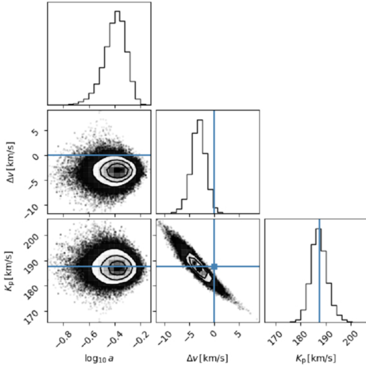
Figure 7. from James T. Sikora et al 2026 Astron. J. 171 doi:10.3847/1538-3881/ae5a29 https://dx.doi.org/10.3847/1538-3881/ae5a29 © 2026. The Author(s). Published by the American Astronomical Society.
