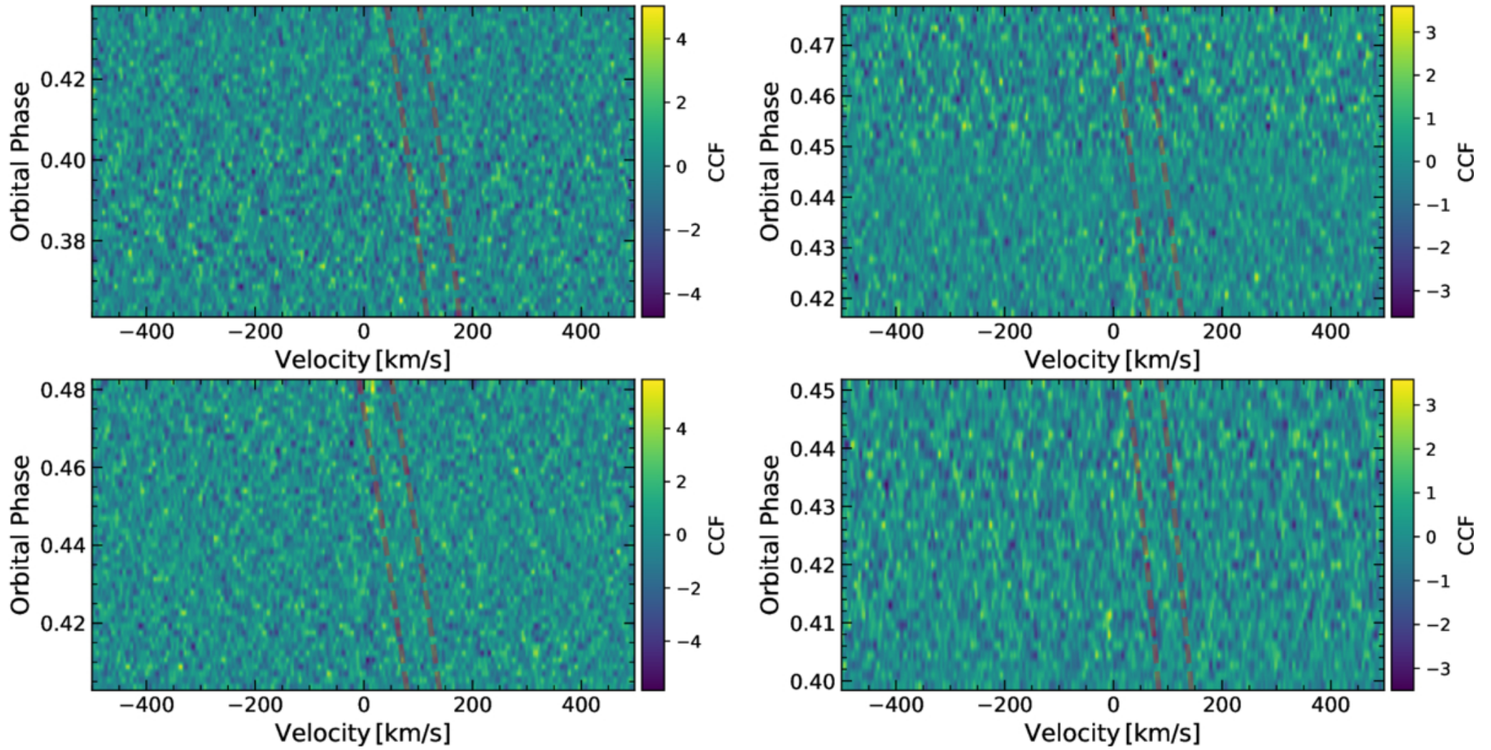
Figure 5. from James T. Sikora et al 2026 Astron. J. 171 doi:10.3847/1538-3881/ae5a29 https://dx.doi.org/10.3847/1538-3881/ae5a29 © 2026. The Author(s). Published by the American Astronomical Society.
