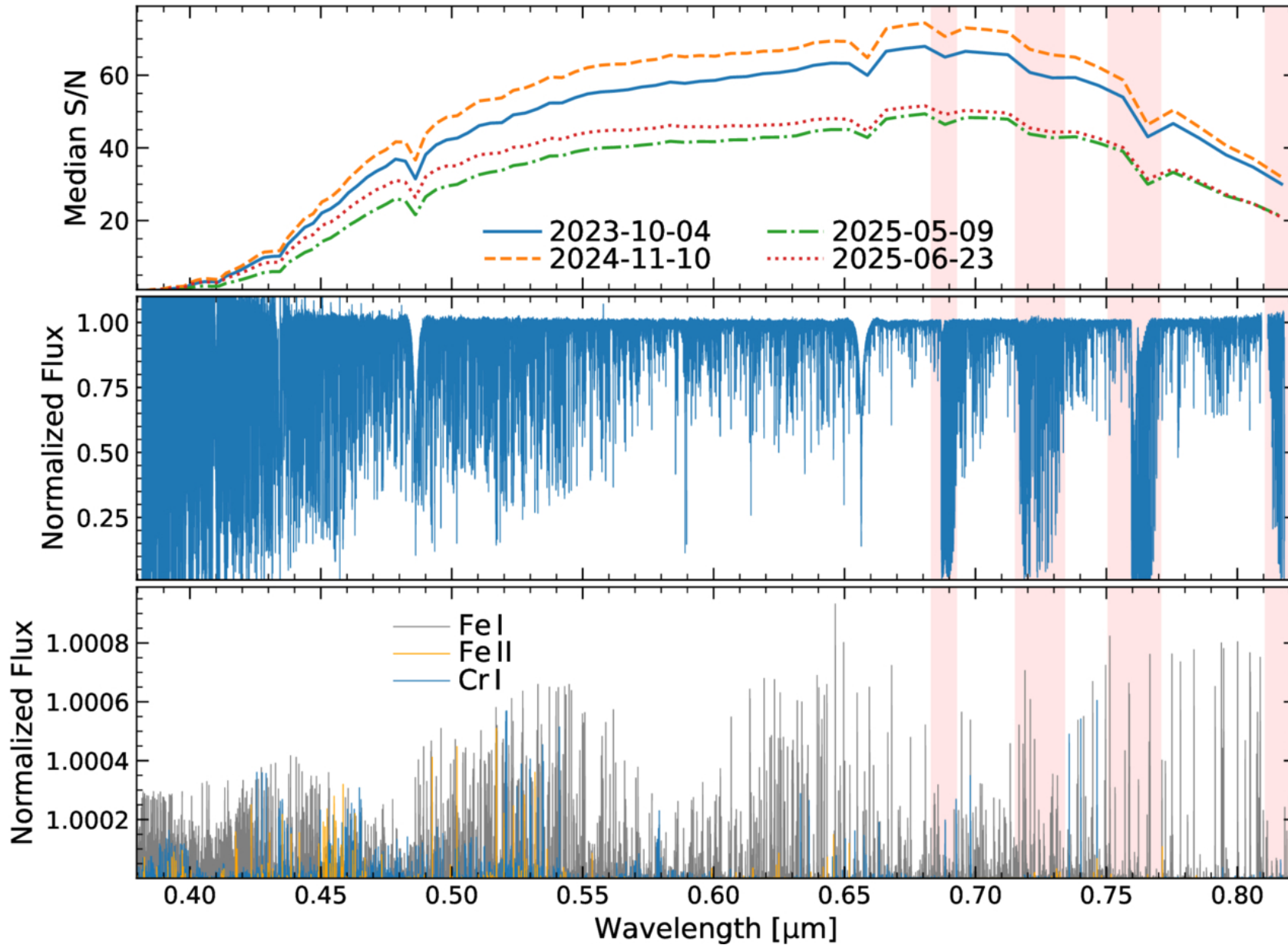
Figure 4. from James T. Sikora et al 2026 Astron. J. 171 doi:10.3847/1538-3881/ae5a29 https://dx.doi.org/10.3847/1538-3881/ae5a29 © 2026. The Author(s). Published by the American Astronomical Society.
