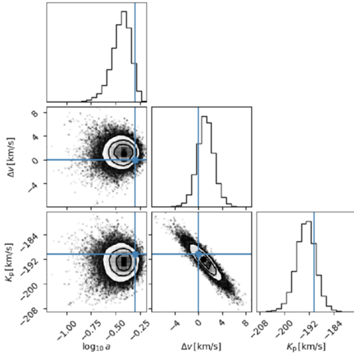
Figure 10. from James T. Sikora et al 2026 Astron. J. 171 doi:10.3847/1538-3881/ae5a29 https://dx.doi.org/10.3847/1538-3881/ae5a29 © 2026. The Author(s). Published by the American Astronomical Society.
