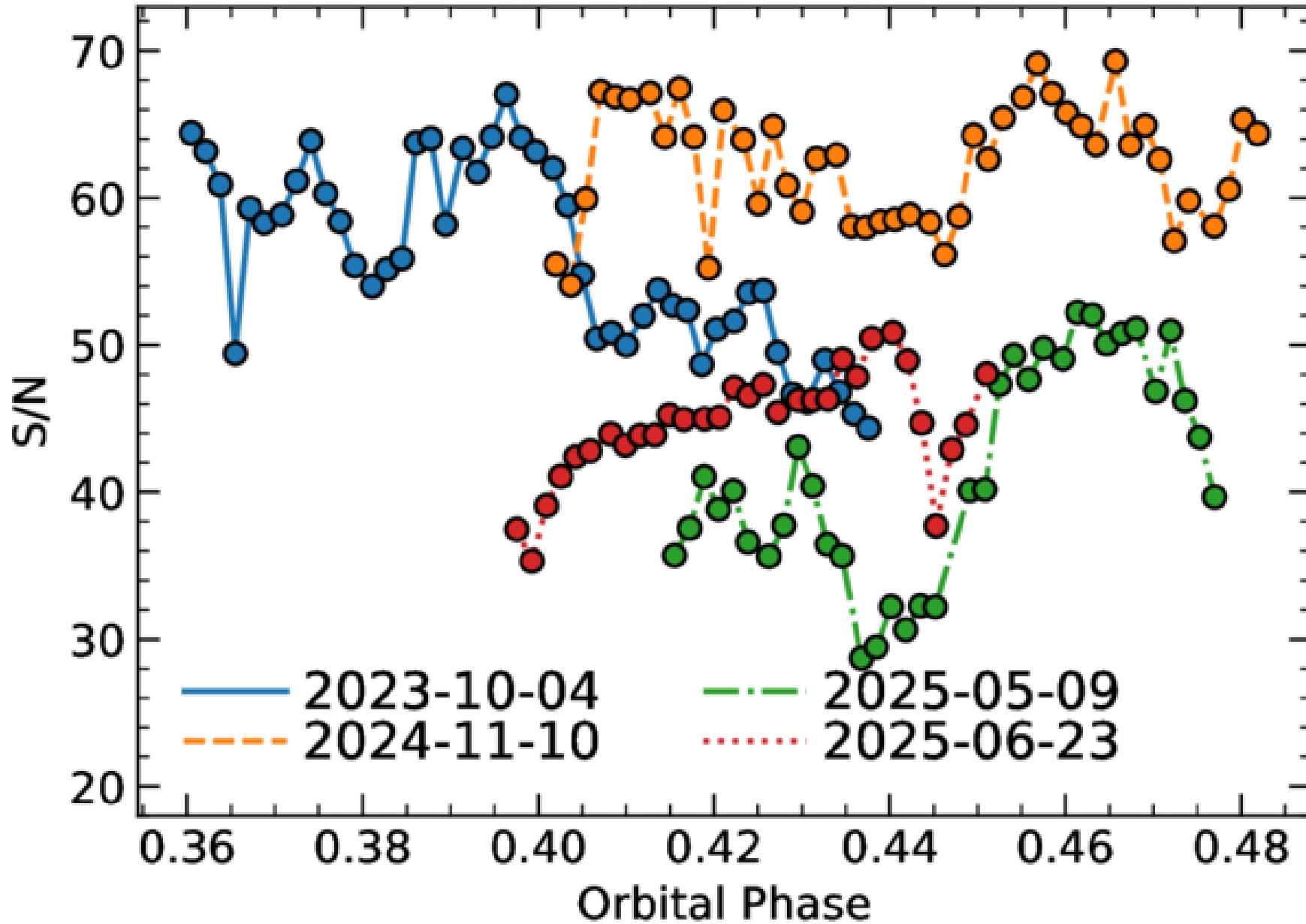
Figure 1. from James T. Sikora et al 2026 Astron. J. 171 doi:10.3847/1538-3881/ae5a29 https://dx.doi.org/10.3847/1538-3881/ae5a29 © 2026. The Author(s). Published by the American Astronomical Society.
