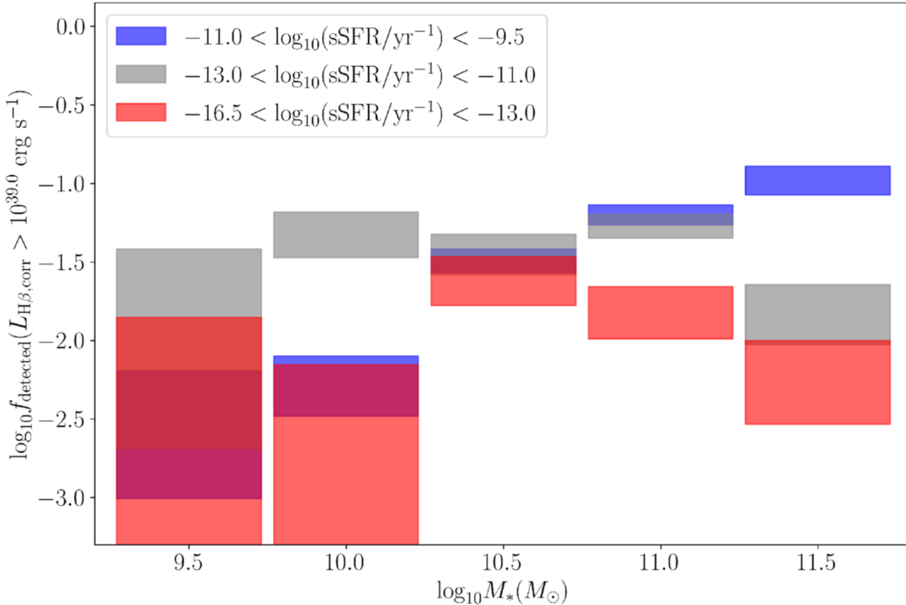
Figure 6. from Michael R. Blanton et al 2026 Astron. J. 171 doi:10.3847/1538-3881/ae5a1e https://dx.doi.org/10.3847/1538-3881/ae5a1e © 2026. The Author(s). Published by the American Astronomical Society.
