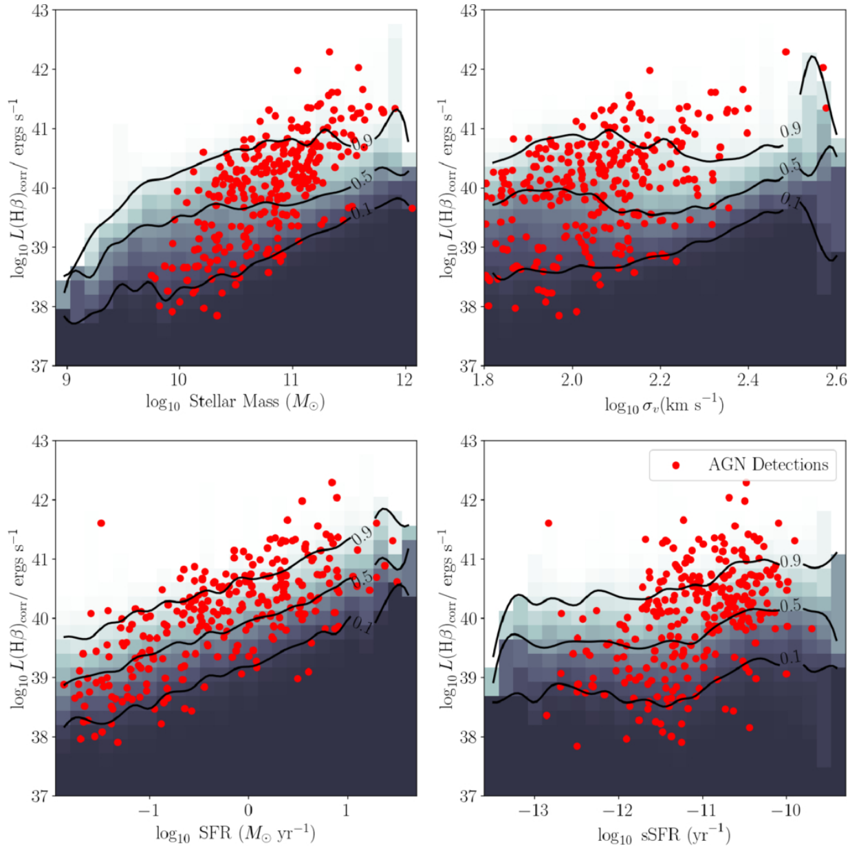
Figure 4. from Michael R. Blanton et al 2026 Astron. J. 171 doi:10.3847/1538-3881/ae5a1e https://dx.doi.org/10.3847/1538-3881/ae5a1e © 2026. The Author(s). Published by the American Astronomical Society.
