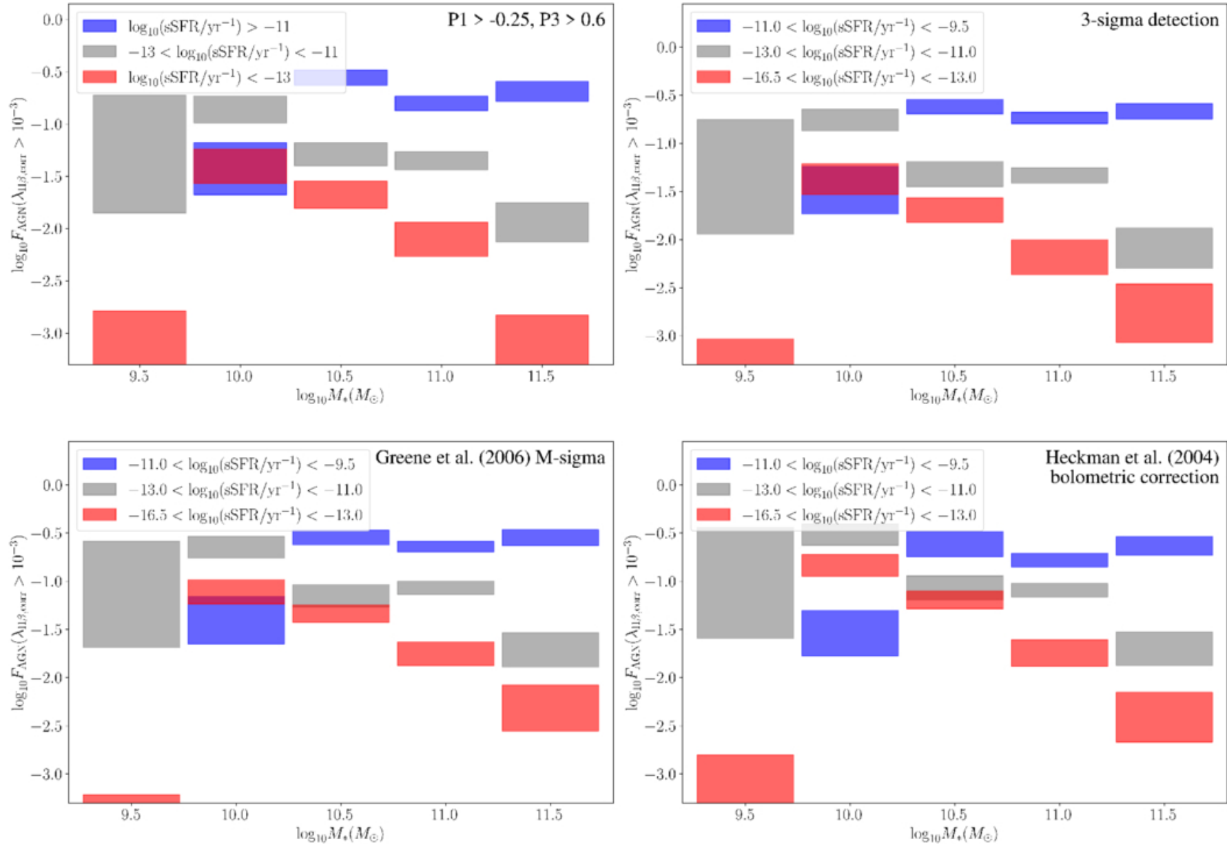
Figure 15. from Michael R. Blanton et al 2026 Astron. J. 171 doi:10.3847/1538-3881/ae5a1e https://dx.doi.org/10.3847/1538-3881/ae5a1e © 2026. The Author(s). Published by the American Astronomical Society.
