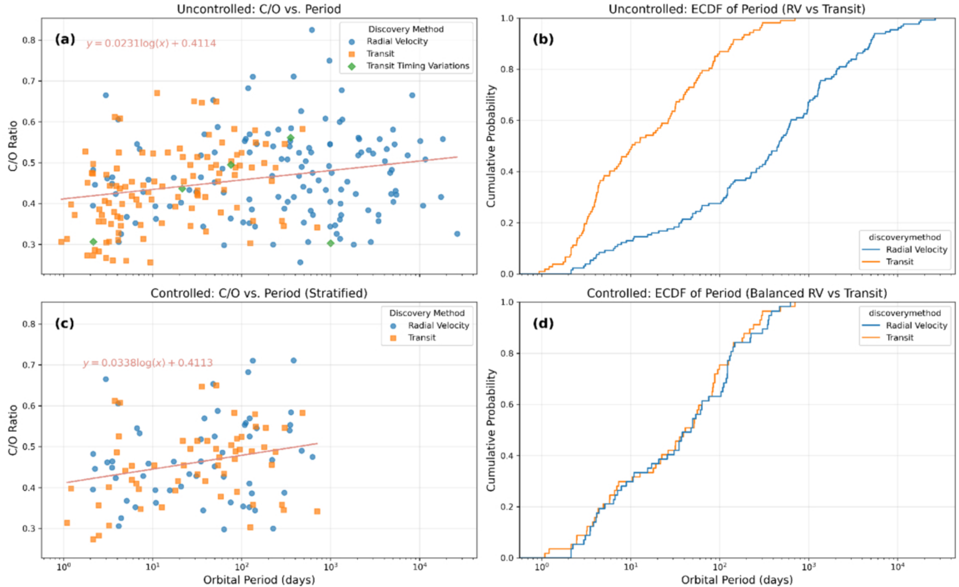
Figure 8. from Ruisheng Zhang et al 2026 Astron. J. 171 doi:10.3847/1538-3881/ae5952 https://dx.doi.org/10.3847/1538-3881/ae5952 © 2026. The Author(s). Published by the American Astronomical Society.
