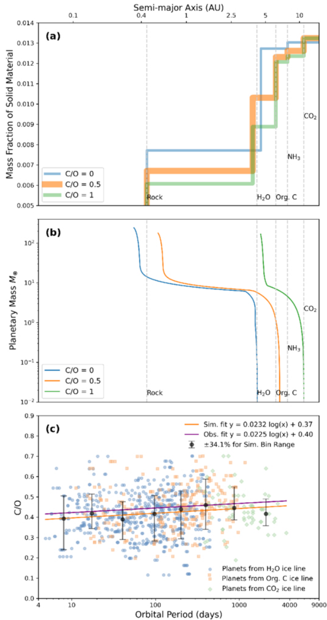
Figure 7. from Ruisheng Zhang et al 2026 Astron. J. 171 doi:10.3847/1538-3881/ae5952 https://dx.doi.org/10.3847/1538-3881/ae5952 © 2026. The Author(s). Published by the American Astronomical Society.
