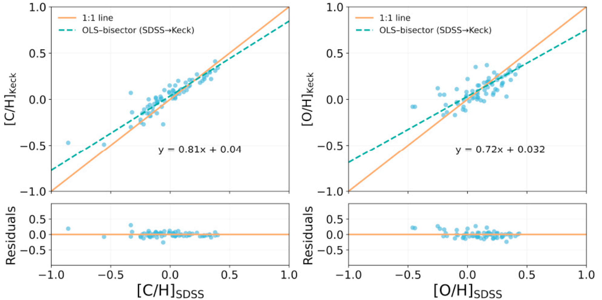
Figure 13. from Ruisheng Zhang et al 2026 Astron. J. 171 doi:10.3847/1538-3881/ae5952 https://dx.doi.org/10.3847/1538-3881/ae5952 © 2026. The Author(s). Published by the American Astronomical Society.
