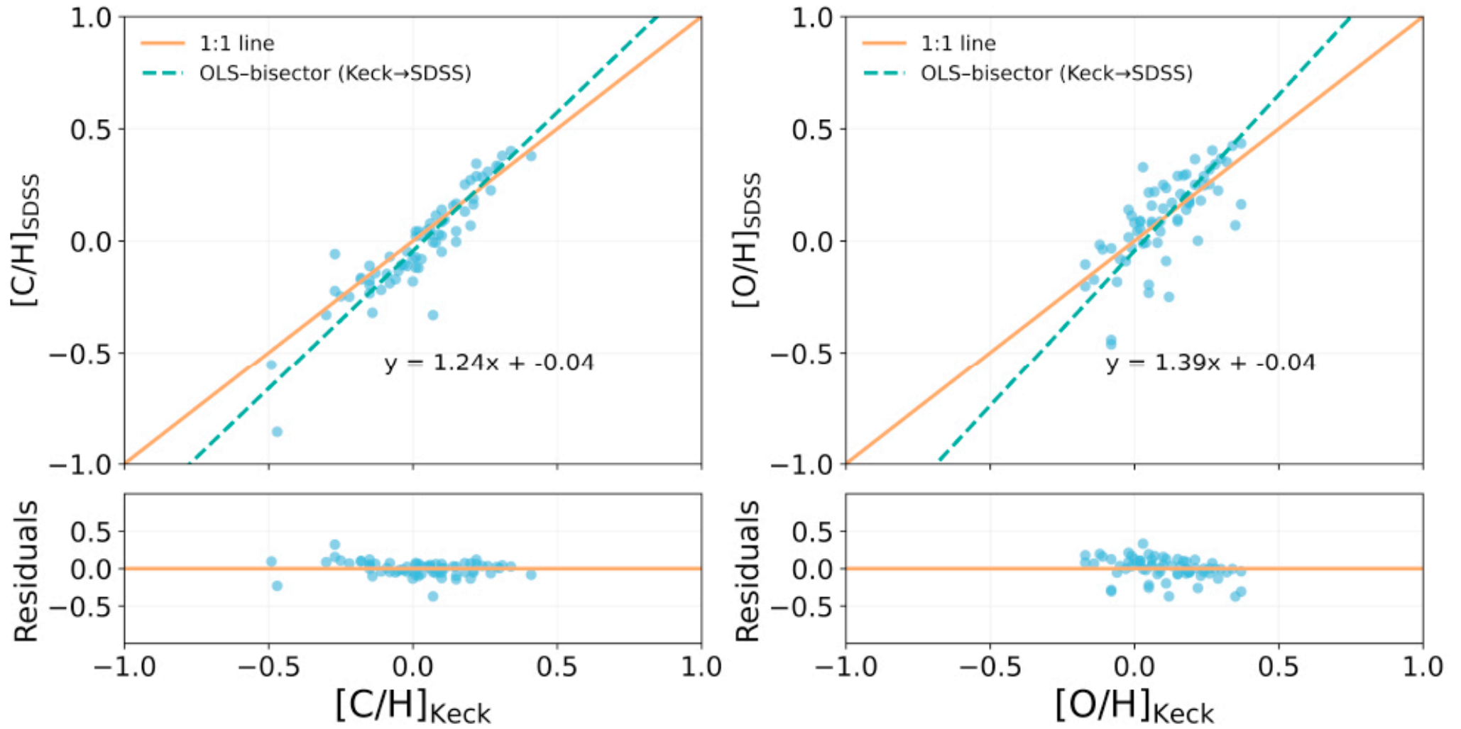
Figure 10. from Ruisheng Zhang et al 2026 Astron. J. 171 doi:10.3847/1538-3881/ae5952 https://dx.doi.org/10.3847/1538-3881/ae5952 © 2026. The Author(s). Published by the American Astronomical Society.
