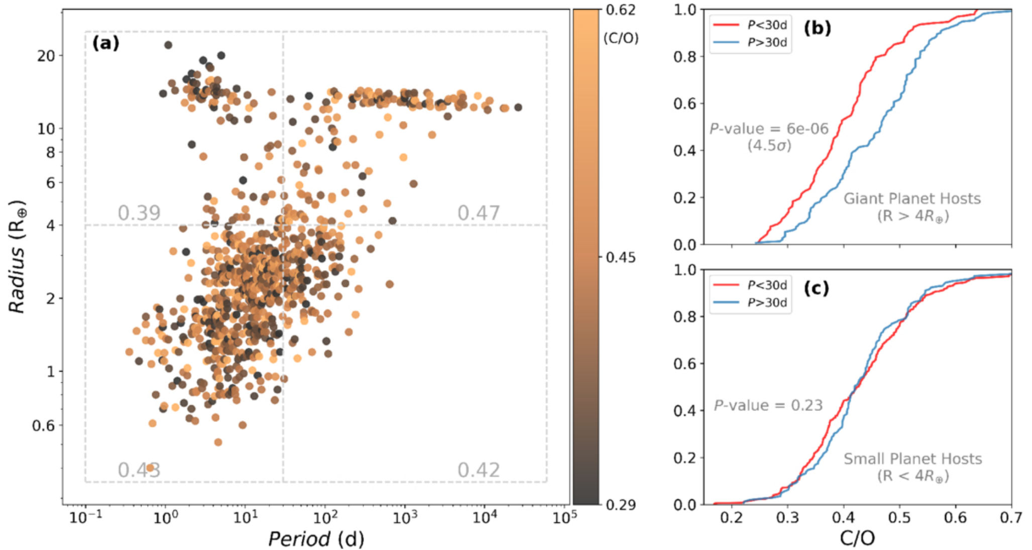
Figure 1. from Ruisheng Zhang et al 2026 Astron. J. 171 doi:10.3847/1538-3881/ae5952 https://dx.doi.org/10.3847/1538-3881/ae5952 © 2026. The Author(s). Published by the American Astronomical Society.
