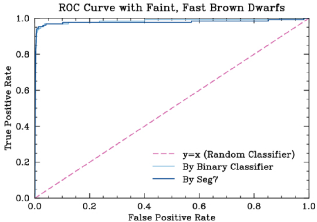
Figure 6. from Dan Caselden et al 2026 Astron. J. 171 doi:10.3847/1538-3881/ae593c https://dx.doi.org/10.3847/1538-3881/ae593c © 2026. The Author(s). Published by the American Astronomical Society.
