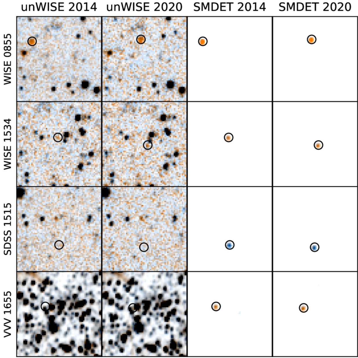
Figure 4. from Dan Caselden et al 2026 Astron. J. 171 doi:10.3847/1538-3881/ae593c https://dx.doi.org/10.3847/1538-3881/ae593c © 2026. The Author(s). Published by the American Astronomical Society.
