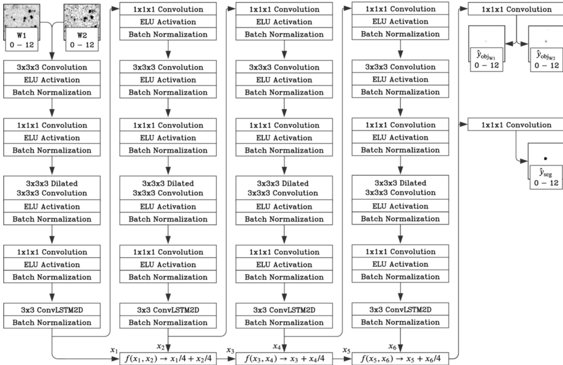
Figure 2. from Dan Caselden et al 2026 Astron. J. 171 doi:10.3847/1538-3881/ae593c https://dx.doi.org/10.3847/1538-3881/ae593c © 2026. The Author(s). Published by the American Astronomical Society.
