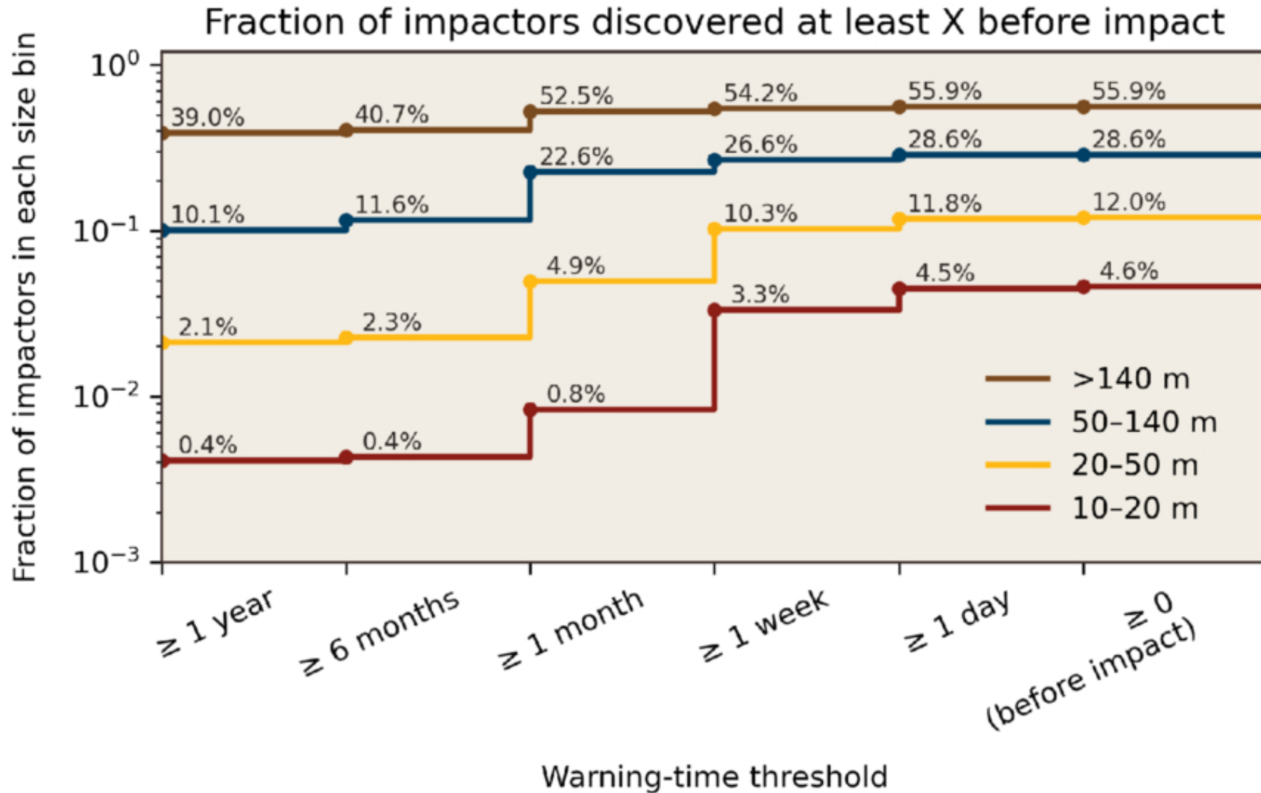
Figure 7. from Qifeng Cheng et al 2026 Astron. J. 171 doi:10.3847/1538-3881/ae5936 https://dx.doi.org/10.3847/1538-3881/ae5936 © 2026. The Author(s). Published by the American Astronomical Society.
