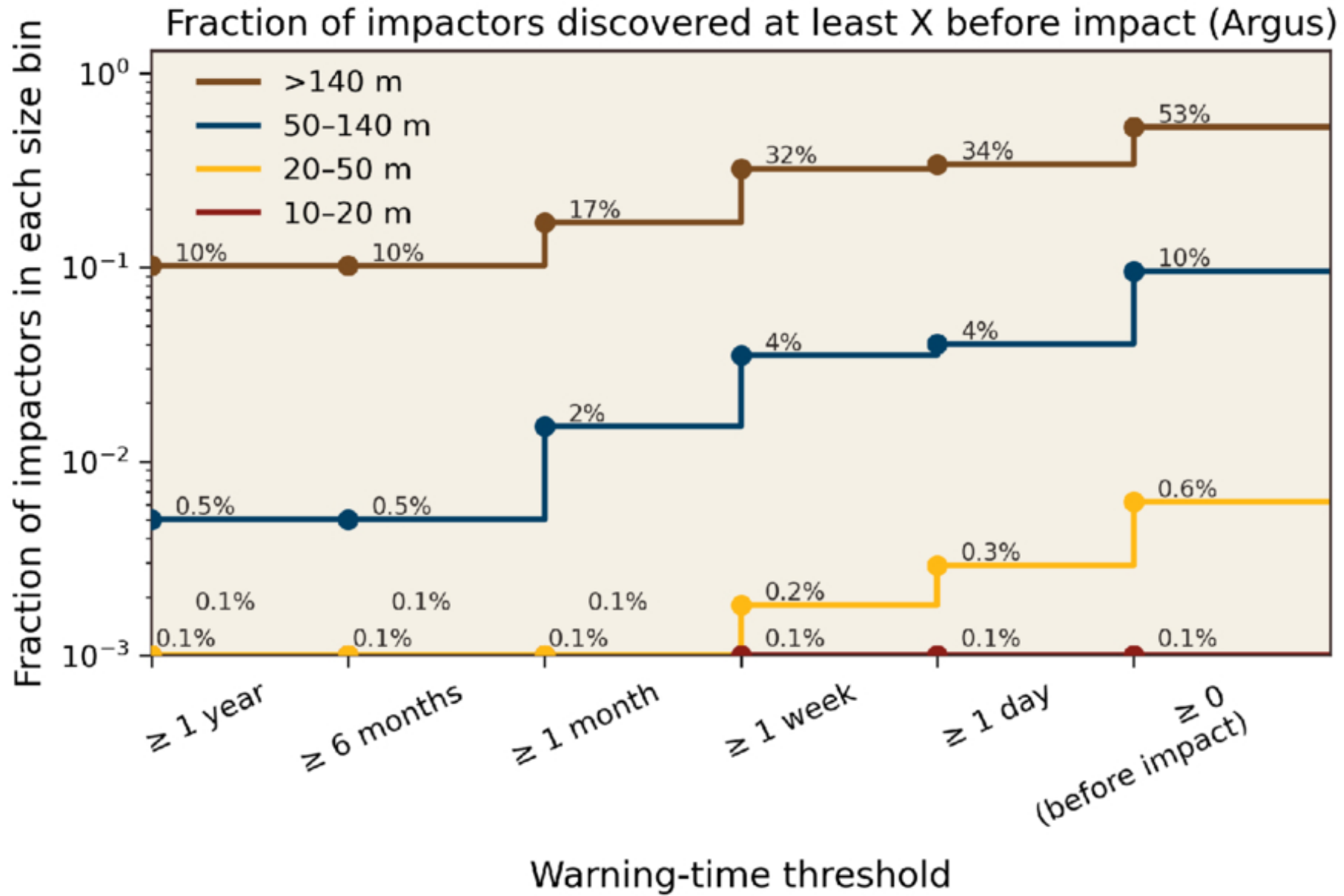
Figure 5. from Qifeng Cheng et al 2026 Astron. J. 171 doi:10.3847/1538-3881/ae5936 https://dx.doi.org/10.3847/1538-3881/ae5936 © 2026. The Author(s). Published by the American Astronomical Society.
