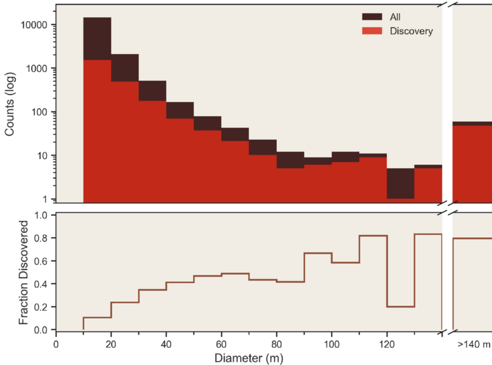
Figure 2. from Qifeng Cheng et al 2026 Astron. J. 171 doi:10.3847/1538-3881/ae5936 https://dx.doi.org/10.3847/1538-3881/ae5936 © 2026. The Author(s). Published by the American Astronomical Society.
