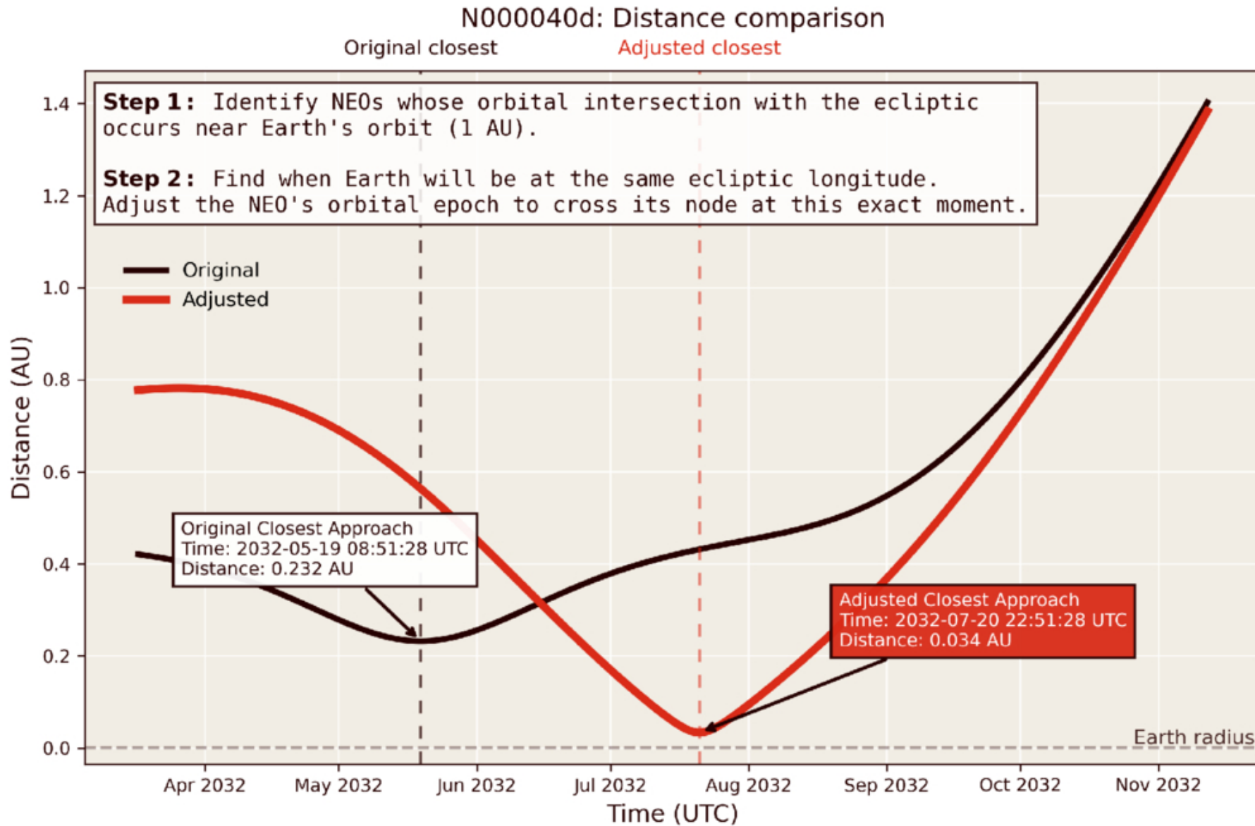
Figure 1. from Qifeng Cheng et al 2026 Astron. J. 171 doi:10.3847/1538-3881/ae5936 https://dx.doi.org/10.3847/1538-3881/ae5936 © 2026. The Author(s). Published by the American Astronomical Society.
