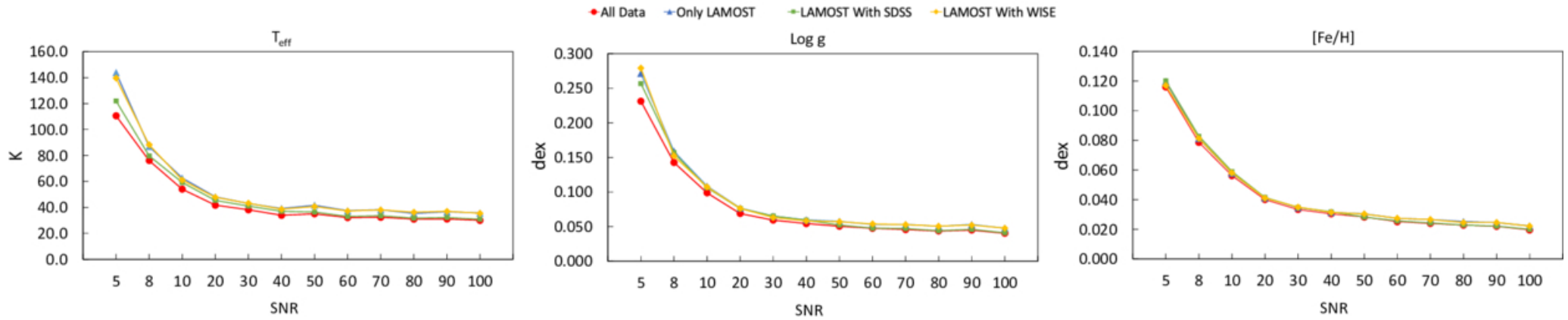
Figure 6. from Jingjing Wu et al 2026 Astron. J. 171 doi:10.3847/1538-3881/ae592f https://dx.doi.org/10.3847/1538-3881/ae592f © 2026. The Author(s). Published by the American Astronomical Society.
