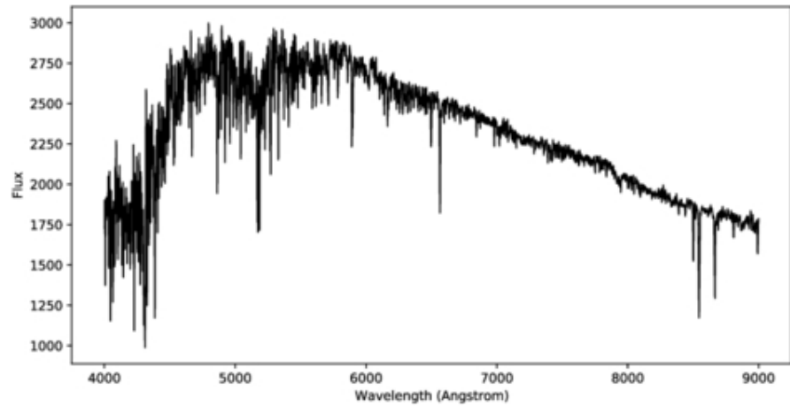
Figure 1. from Jingjing Wu et al 2026 Astron. J. 171 doi:10.3847/1538-3881/ae592f https://dx.doi.org/10.3847/1538-3881/ae592f © 2026. The Author(s). Published by the American Astronomical Society.
