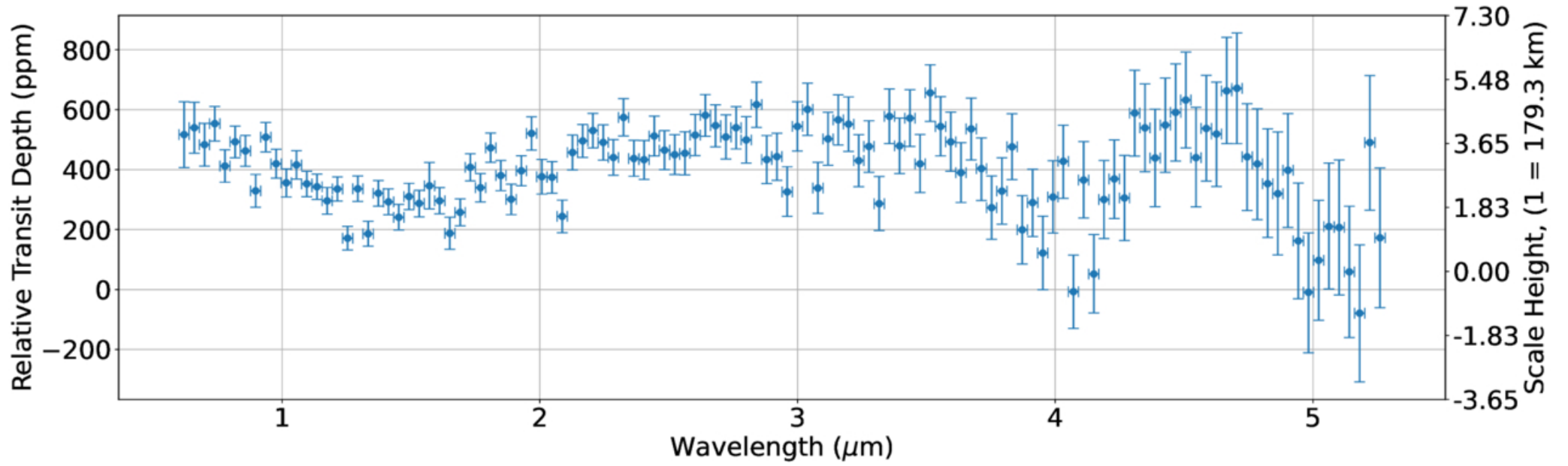
Figure 5. from Reza Ashtari et al 2026 Astron. J. 171 doi:10.3847/1538-3881/ae552c https://dx.doi.org/10.3847/1538-3881/ae552c © 2026. The Author(s). Published by the American Astronomical Society.
