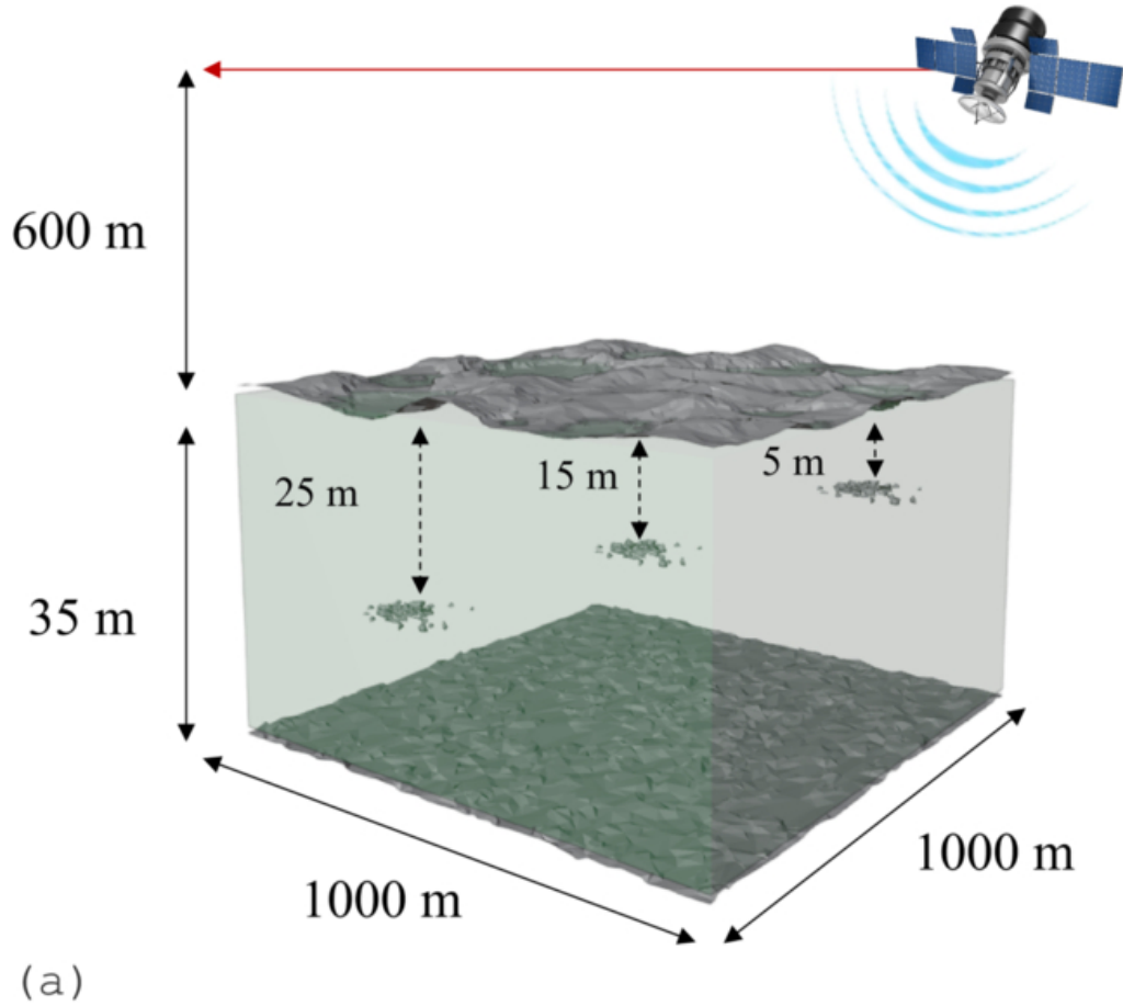
Figure 4. from Wei Guan et al 2026 Astron. J. 171 doi:10.3847/1538-3881/ae5525 https://dx.doi.org/10.3847/1538-3881/ae5525 © 2026. The Author(s). Published by the American Astronomical Society.
