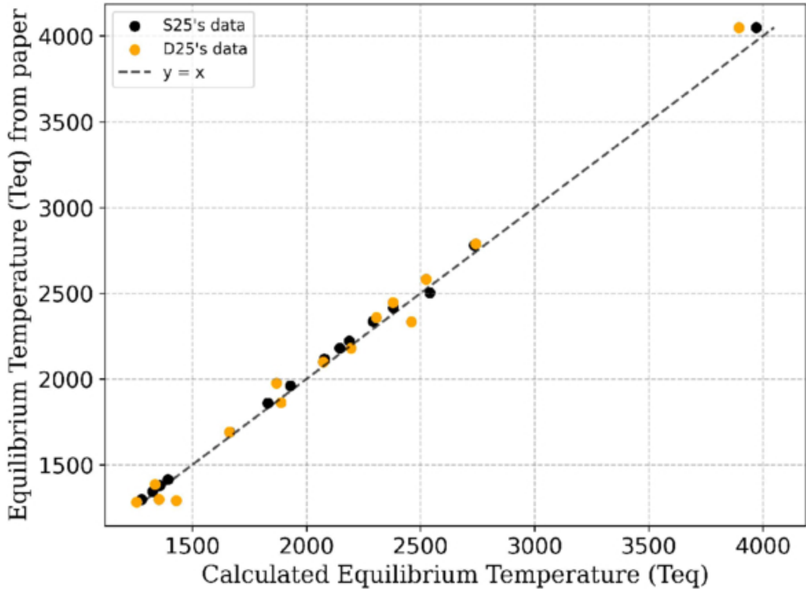
Figure 4. from Emeline Decocq et al 2026 Astron. J. 171 doi:10.3847/1538-3881/ae5486 https://dx.doi.org/10.3847/1538-3881/ae5486 © 2026. The Author(s). Published by the American Astronomical Society.
