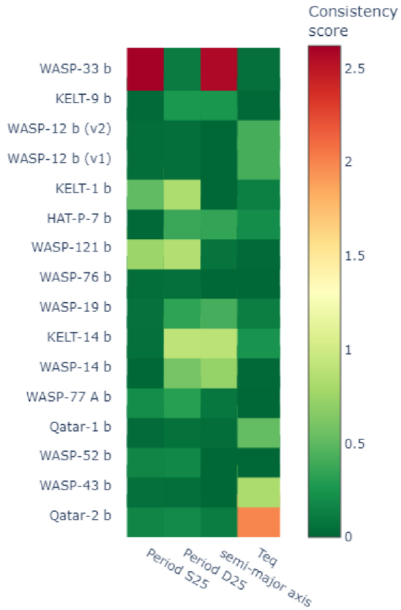
Figure 3. from Emeline Decocq et al 2026 Astron. J. 171 doi:10.3847/1538-3881/ae5486 https://dx.doi.org/10.3847/1538-3881/ae5486 © 2026. The Author(s). Published by the American Astronomical Society.
