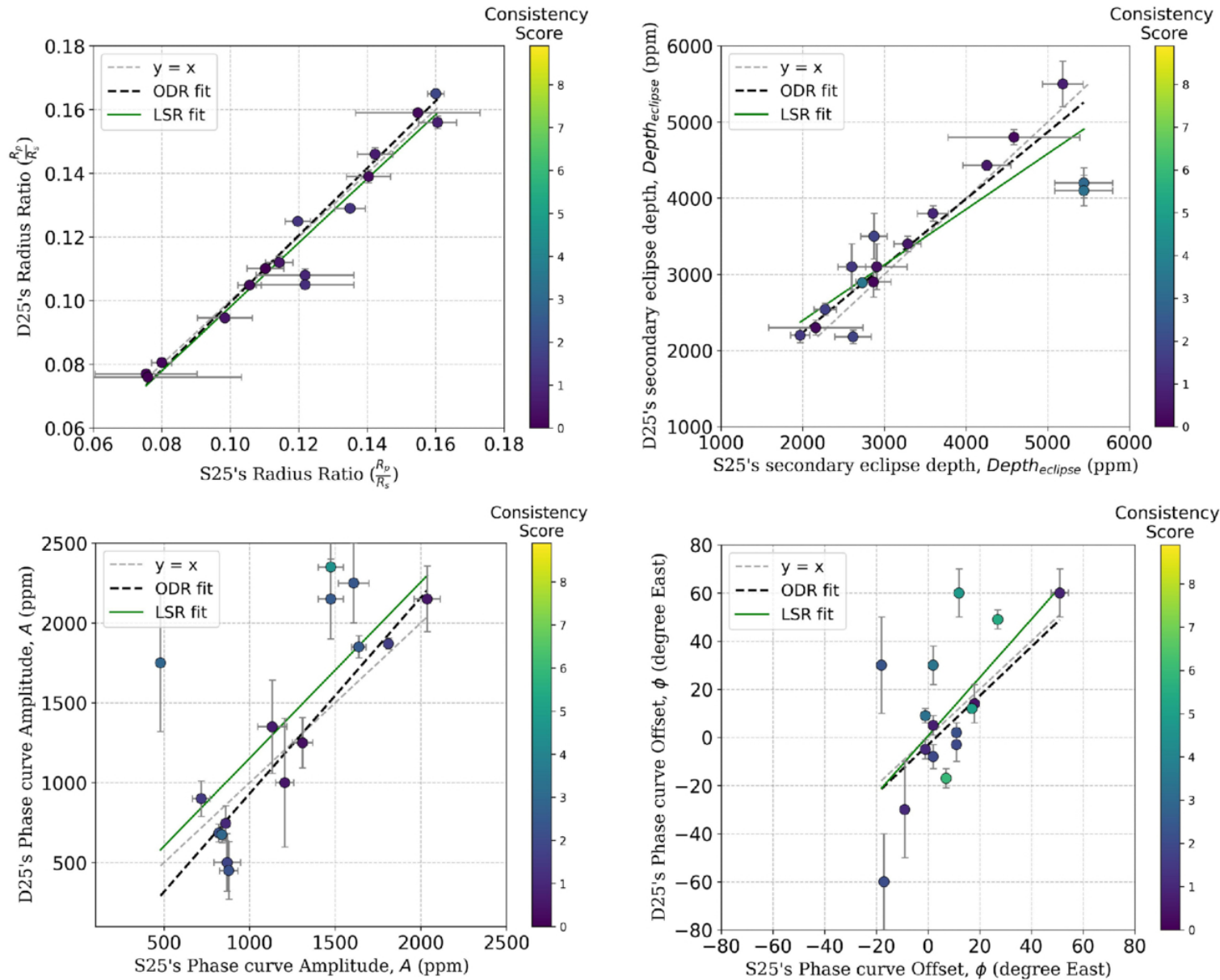
Figure 1. from Emeline Decocq et al 2026 Astron. J. 171 doi:10.3847/1538-3881/ae5486 https://dx.doi.org/10.3847/1538-3881/ae5486 © 2026. The Author(s). Published by the American Astronomical Society.
