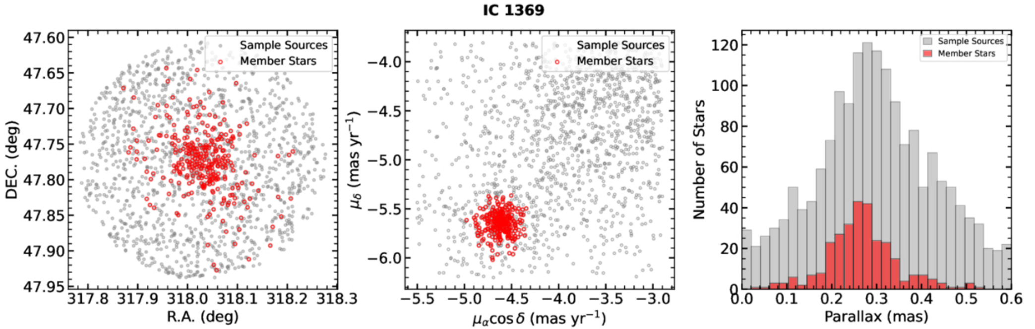
Figure 3. from K. Belwal et al 2026 Astron. J. 171 doi:10.3847/1538-3881/ae53e7 https://dx.doi.org/10.3847/1538-3881/ae53e7 © 2026. The Author(s). Published by the American Astronomical Society.
