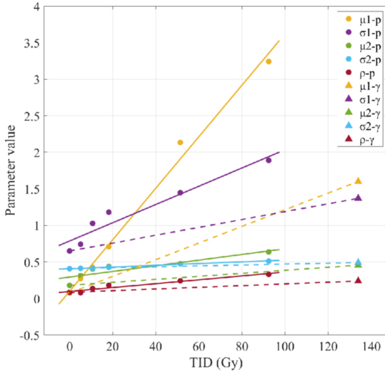
Figure 10. from Qi Feng et al 2026 Astron. J. 171 doi:10.3847/1538-3881/ae522b https://dx.doi.org/10.3847/1538-3881/ae522b © 2026. The Author(s). Published by the American Astronomical Society.
