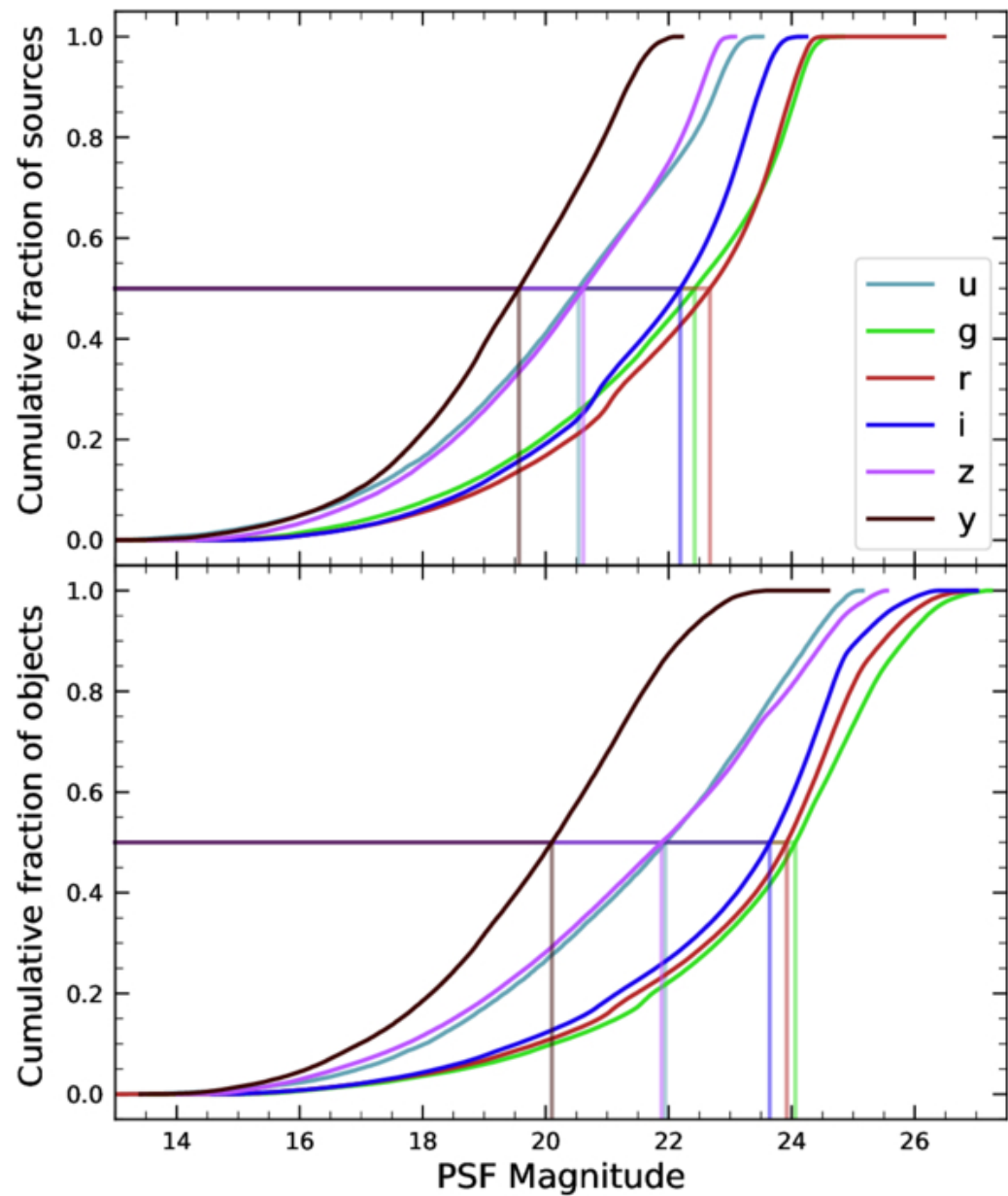
Figure 9. from Tatiana Acero-Cuellar et al 2026 Astron. J. 171 doi:10.3847/1538-3881/ae521f https://dx.doi.org/10.3847/1538-3881/ae521f © 2026. The Author(s). Published by the American Astronomical Society.
