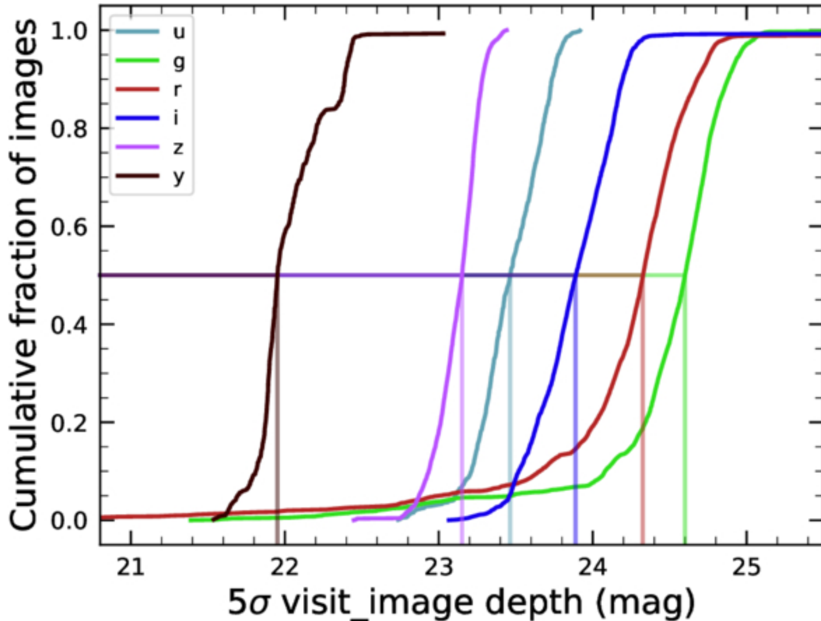
Figure 8. from Tatiana Acero-Cuellar et al 2026 Astron. J. 171 doi:10.3847/1538-3881/ae521f https://dx.doi.org/10.3847/1538-3881/ae521f © 2026. The Author(s). Published by the American Astronomical Society.
