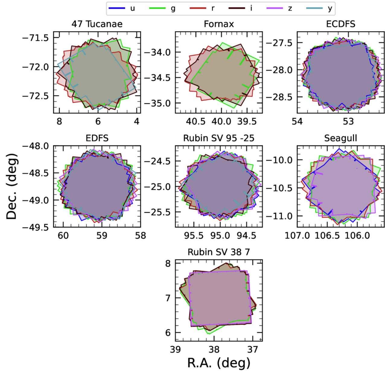
Figure 6. from Tatiana Acero-Cuellar et al 2026 Astron. J. 171 doi:10.3847/1538-3881/ae521f https://dx.doi.org/10.3847/1538-3881/ae521f © 2026. The Author(s). Published by the American Astronomical Society.
