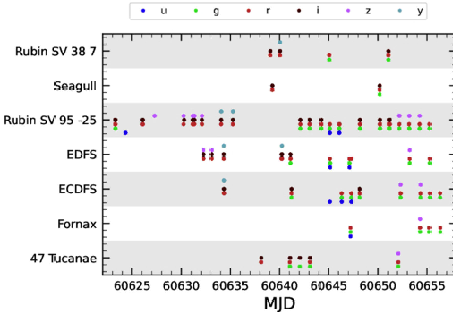
Figure 5. from Tatiana Acero-Cuellar et al 2026 Astron. J. 171 doi:10.3847/1538-3881/ae521f https://dx.doi.org/10.3847/1538-3881/ae521f © 2026. The Author(s). Published by the American Astronomical Society.
