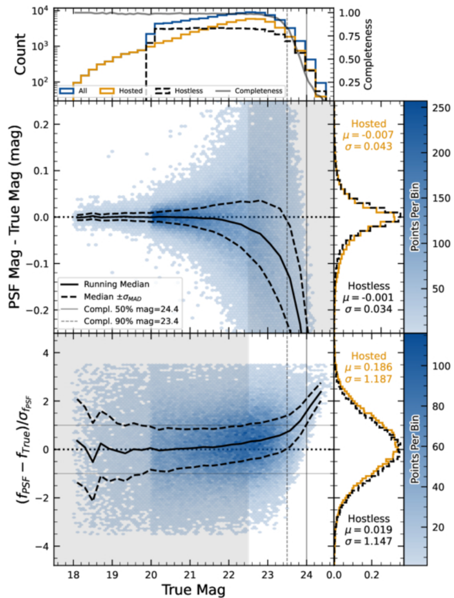
Figure 39. from Tatiana Acero-Cuellar et al 2026 Astron. J. 171 doi:10.3847/1538-3881/ae521f https://dx.doi.org/10.3847/1538-3881/ae521f © 2026. The Author(s). Published by the American Astronomical Society.
