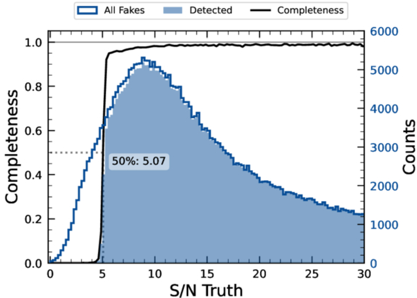
Figure 37. from Tatiana Acero-Cuellar et al 2026 Astron. J. 171 doi:10.3847/1538-3881/ae521f https://dx.doi.org/10.3847/1538-3881/ae521f © 2026. The Author(s). Published by the American Astronomical Society.
