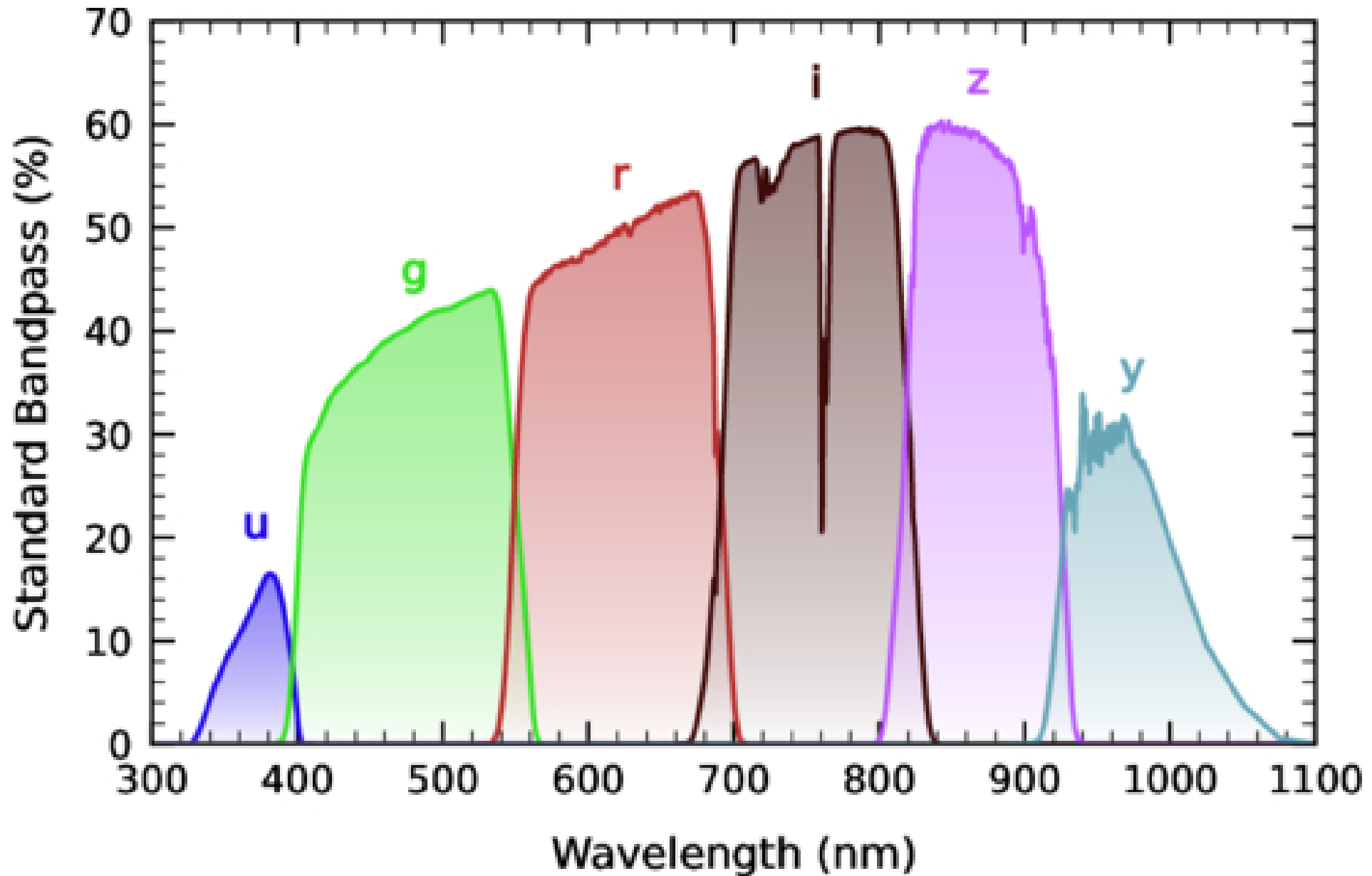
Figure 3. from Tatiana Acero-Cuellar et al 2026 Astron. J. 171 doi:10.3847/1538-3881/ae521f https://dx.doi.org/10.3847/1538-3881/ae521f © 2026. The Author(s). Published by the American Astronomical Society.
