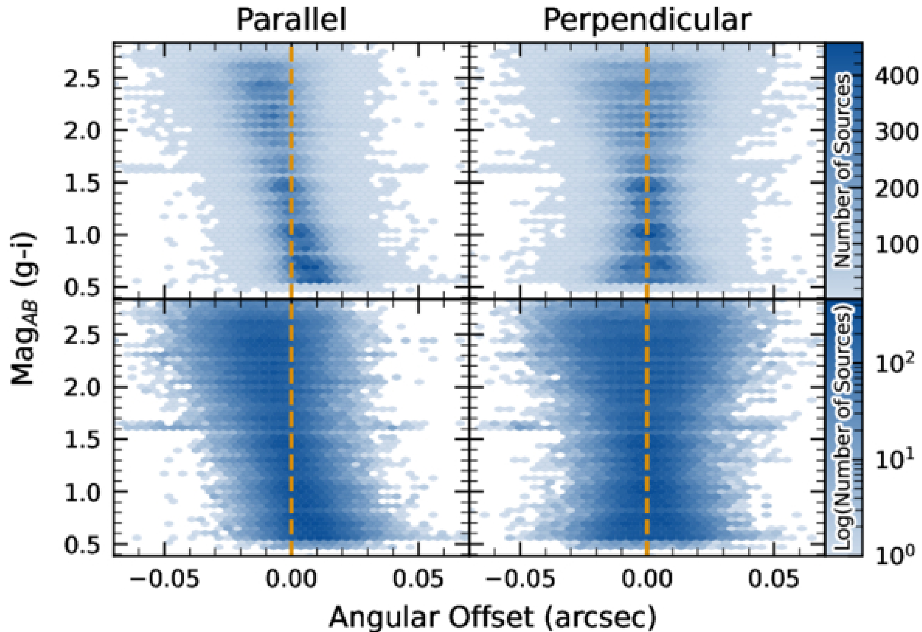
Figure 26. from Tatiana Acero-Cuellar et al 2026 Astron. J. 171 doi:10.3847/1538-3881/ae521f https://dx.doi.org/10.3847/1538-3881/ae521f © 2026. The Author(s). Published by the American Astronomical Society.
