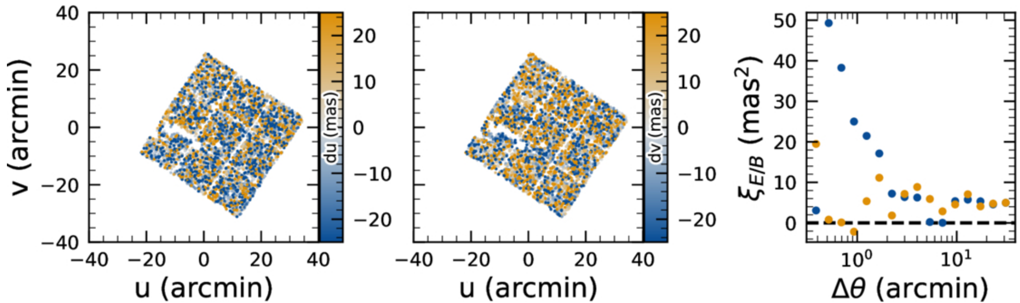
Figure 23. from Tatiana Acero-Cuellar et al 2026 Astron. J. 171 doi:10.3847/1538-3881/ae521f https://dx.doi.org/10.3847/1538-3881/ae521f © 2026. The Author(s). Published by the American Astronomical Society.
