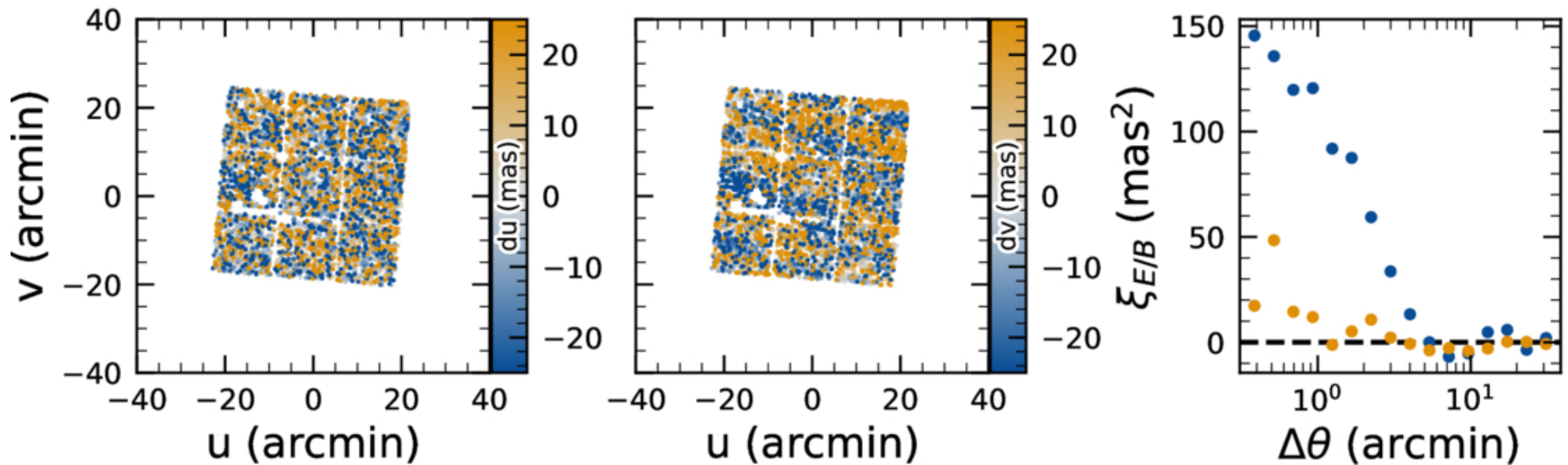
Figure 22. from Tatiana Acero-Cuellar et al 2026 Astron. J. 171 doi:10.3847/1538-3881/ae521f https://dx.doi.org/10.3847/1538-3881/ae521f © 2026. The Author(s). Published by the American Astronomical Society.
