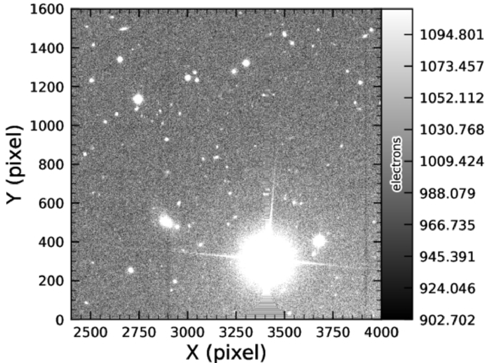
Figure 14. from Tatiana Acero-Cuellar et al 2026 Astron. J. 171 doi:10.3847/1538-3881/ae521f https://dx.doi.org/10.3847/1538-3881/ae521f © 2026. The Author(s). Published by the American Astronomical Society.
