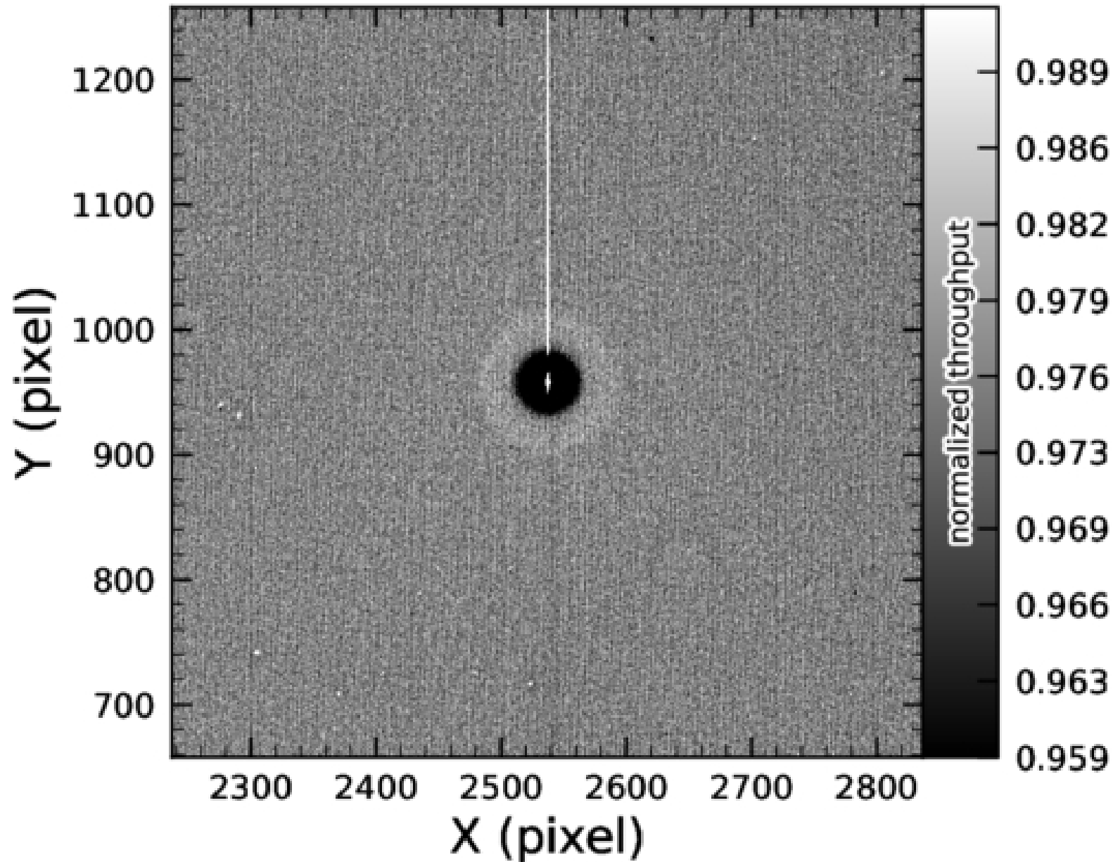
Figure 12. from Tatiana Acero-Cuellar et al 2026 Astron. J. 171 doi:10.3847/1538-3881/ae521f https://dx.doi.org/10.3847/1538-3881/ae521f © 2026. The Author(s). Published by the American Astronomical Society.
