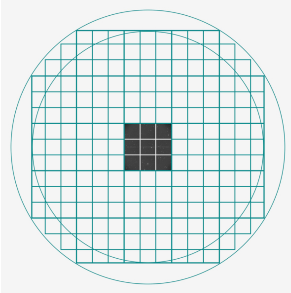
Figure 1. from Tatiana Acero-Cuellar et al 2026 Astron. J. 171 doi:10.3847/1538-3881/ae521f https://dx.doi.org/10.3847/1538-3881/ae521f © 2026. The Author(s). Published by the American Astronomical Society.
