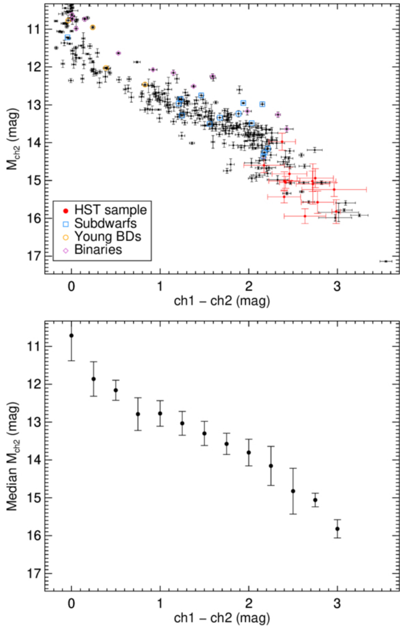
Figure 4. from Federico Marocco et al 2026 Astron. J. 171 doi:10.3847/1538-3881/ae5061 https://dx.doi.org/10.3847/1538-3881/ae5061 © 2026. The Author(s). Published by the American Astronomical Society.
