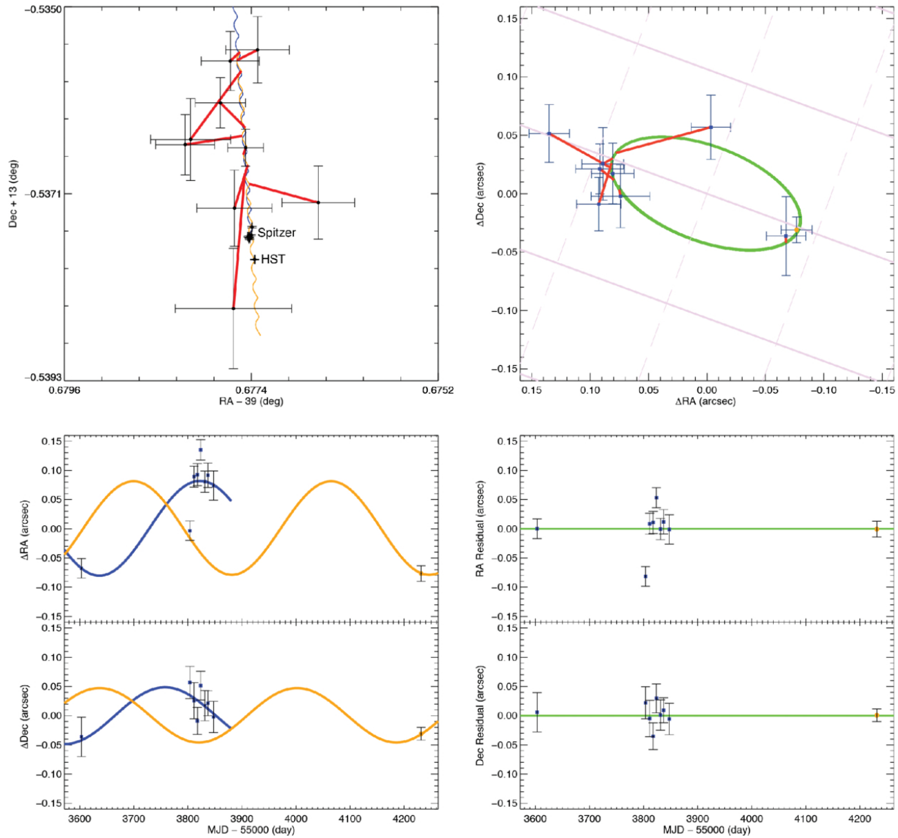
Figure 2. from Federico Marocco et al 2026 Astron. J. 171 doi:10.3847/1538-3881/ae5061 https://dx.doi.org/10.3847/1538-3881/ae5061 © 2026. The Author(s). Published by the American Astronomical Society.
