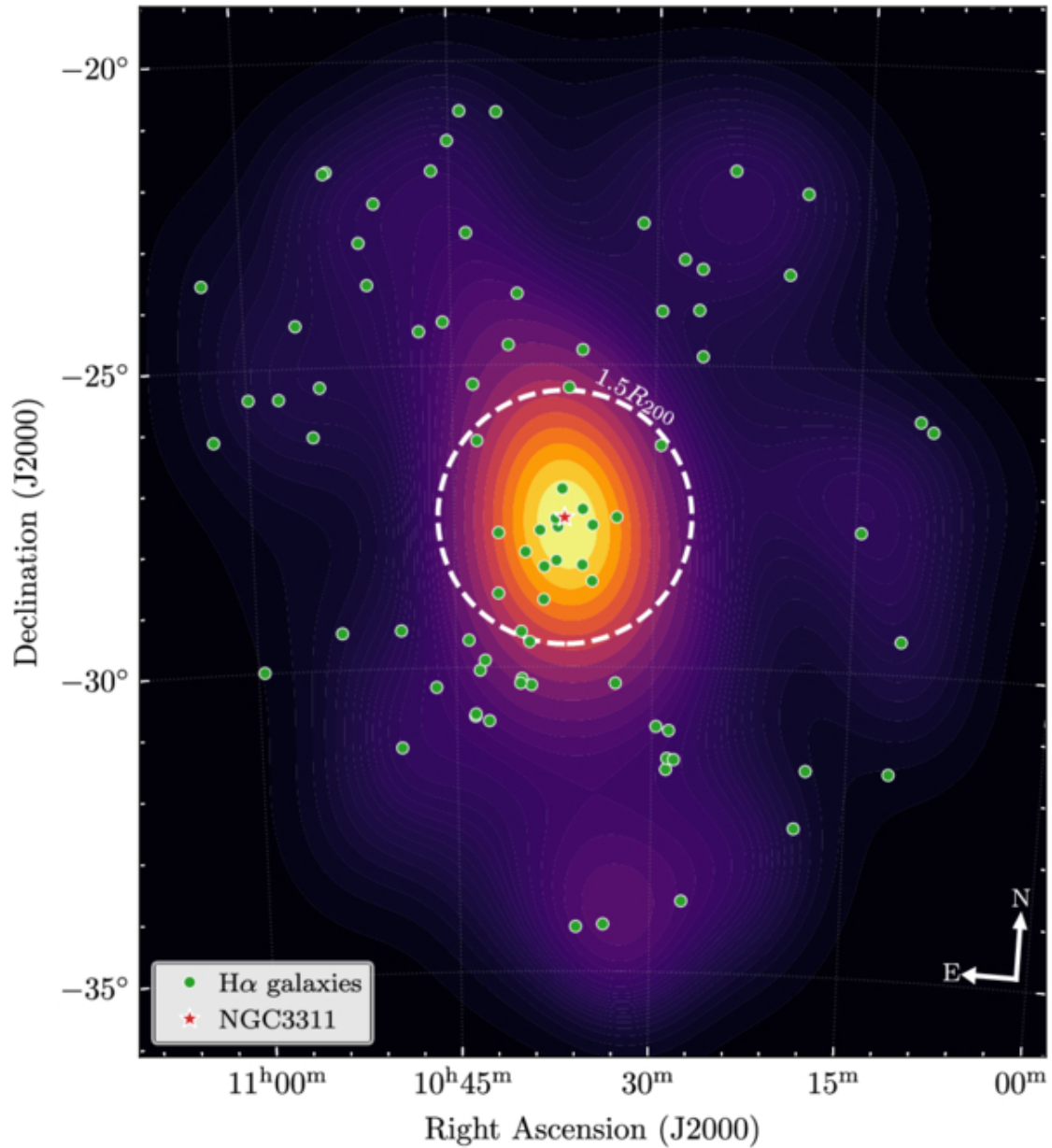
Figure 7. from Natanael M. Cardoso et al 2026 Astron. J. 171 doi:10.3847/1538-3881/ae4fb1 https://dx.doi.org/10.3847/1538-3881/ae4fb1 © 2026. The Author(s). Published by the American Astronomical Society.
