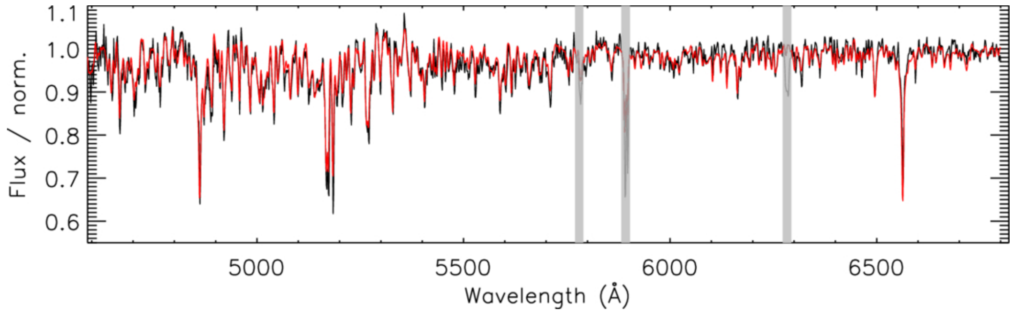
Figure 9. from Yoon-Hyun Ryu et al 2026 Astron. J. 171 doi:10.3847/1538-3881/ae4edf https://dx.doi.org/10.3847/1538-3881/ae4edf © 2026. The Author(s). Published by the American Astronomical Society.
