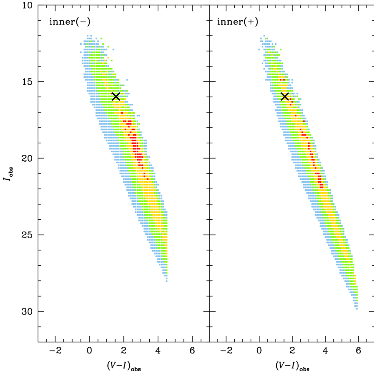
Figure 8. from Yoon-Hyun Ryu et al 2026 Astron. J. 171 doi:10.3847/1538-3881/ae4edf https://dx.doi.org/10.3847/1538-3881/ae4edf © 2026. The Author(s). Published by the American Astronomical Society.
